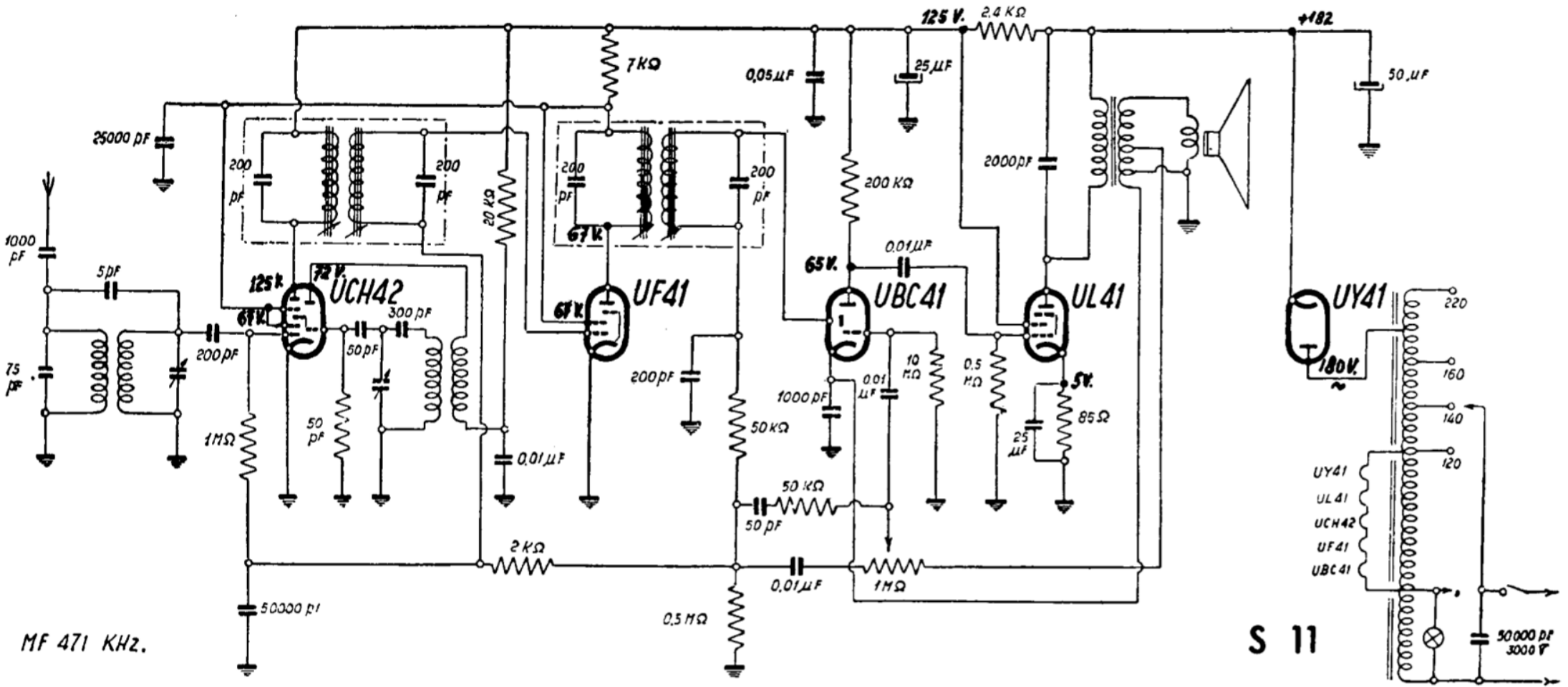
MAGNADYNE RADIO - Mod. S 11. Gamma onde medie. Media frequenza 471 kc/s.
